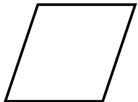
parallelogram
