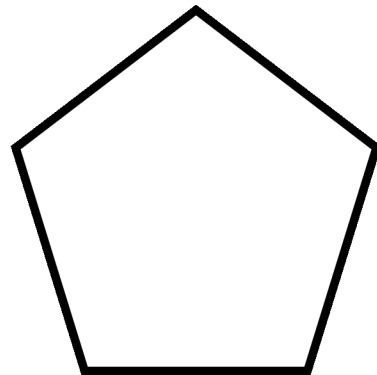
pentagon
