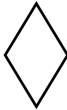
diamond
